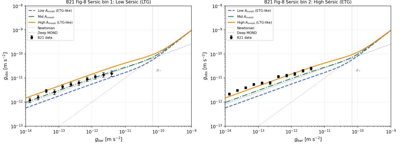
FIG. 7. WT lensing RAR prediction by A_{\text{morph}} tertile, overlaid on Brouwer et al. (2021) KiDS-1000 Sérsic-split measurements. Left: B21 Sérsic bin 1 (low Sérsic index, LTG); right: B21 Sérsic bin 2 (high Sérsic index, ETG). Coloured curves show the WT prediction g_{\text{obs}}(g_{\text{bar}}) for low ( \alpha_0 = 0.694 , blue dashed), mid ( \alpha_0 = 1.178 , green dash-dot), and high ( \alpha_0 = 1.804 , orange solid) A_{\text{morph}} tertiles. Reference lines show the Newtonian relation (dotted) and deep-MOND scaling (dashed grey). The WT curves bracket the data with the correct ordering. The amplitude offset ( \sim 3\text{--}5\times ) reflects gas-fraction incompleteness in the B21 stellar-mass estimate of g_{\text{bar}} (see text).
