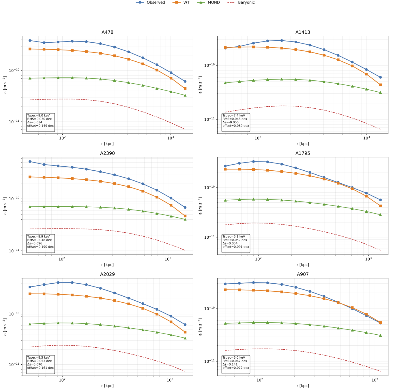
FIG. 6. Six best-matching clusters for the exploratory suppressed extension, shown for the global parameter choice \alpha_{\text{cl}} = 9 and M_{\text{gal}} = 5 \times 10^{11} M_{\odot} ( r_{\text{bal}} \simeq 978 kpc). Blue: observed acceleration from Vikhlinin et al. [16] hydrostatic masses. Orange: suppressed WT profile (eq. 120). Green: MOND (McGaugh interpolation function). Red dashed: baryonic (gas) contribution. Insets report T_{\text{spec}} , normalisation-free shape RMS, slope mismatch \Delta s = s_{\text{WT}} - s_{\text{obs}} , and mean logarithmic offset. All six systems show shape errors \text{RMS}_{\text{shape}} < 0.07 dex; residual discrepancies are primarily in amplitude rather than radial form.
